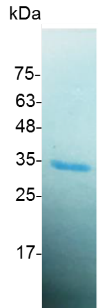
SDS-PAGE analysis of recombinant human HMGB1
